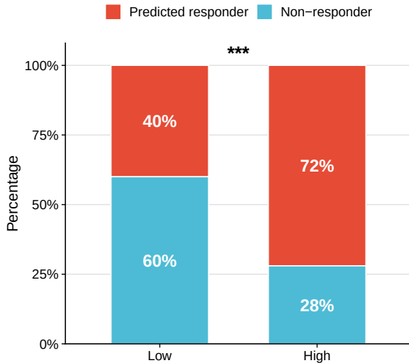
LAML TIDE-predicted response
